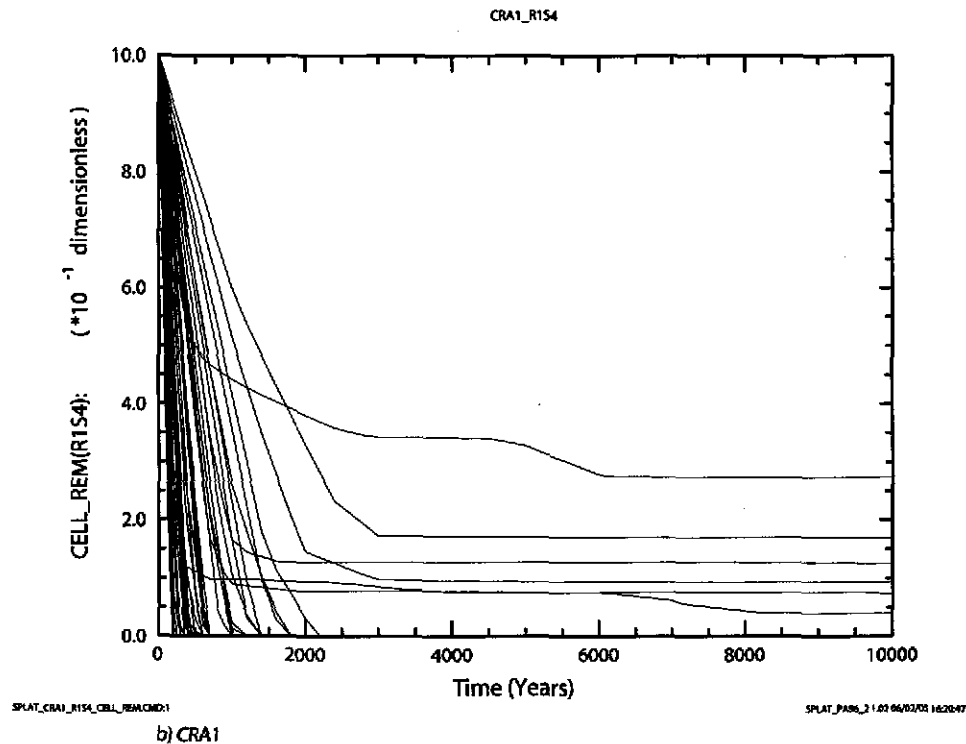
Figure 6-50. Fraction of cellulose (dimensionless) remaining versus time (years) for all 100 vectors in Replicate 1, Scenario S4. Fraction of cellulose is either cellulose or CPR depending on the value of WAS_AREA:PROBDEG ($5.4). Figure a) shows results from the CRA-2004 PABC. Figure b) shows results from the CRA-2004.
