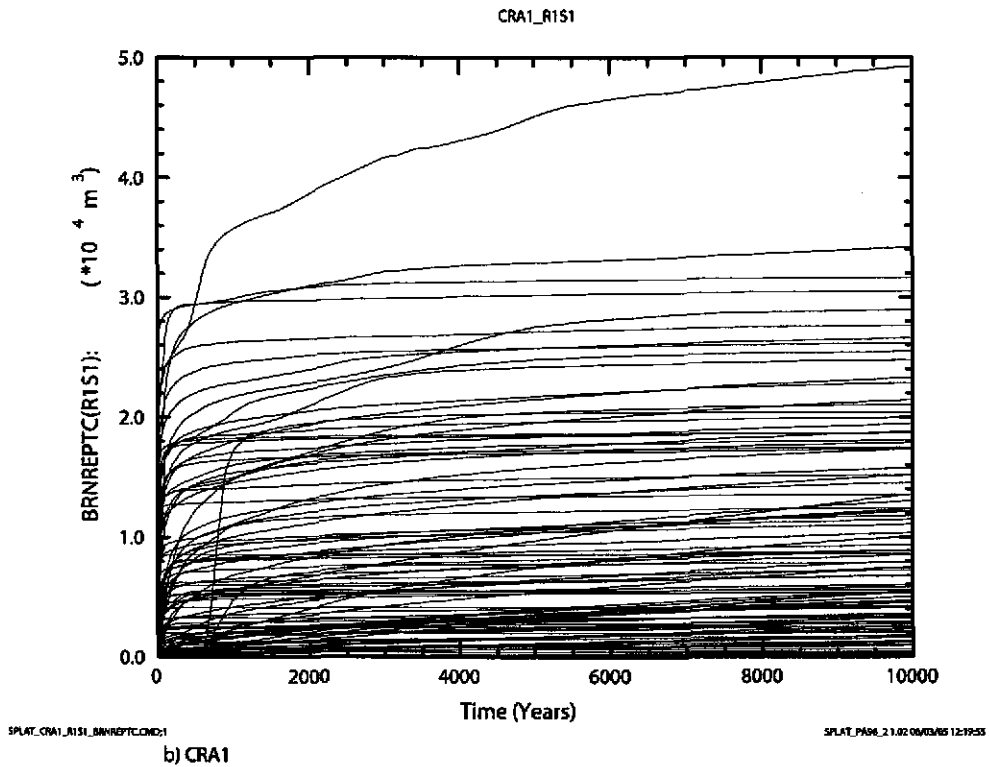
Figure 6-2. Total cumulative inflow of brine ( m^3 ) into the repository versus time (years) for all 100 vectors in Replicate 1, Scenario S1. Figure a) shows results from the CRA-2004 PABC. Figure b) shows results from the CRA-2004.
