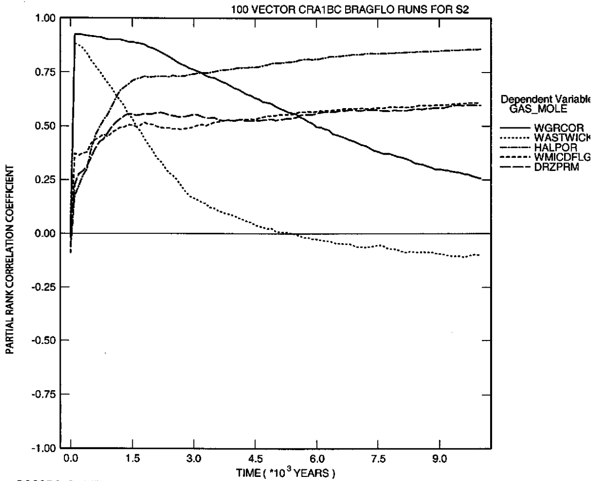
Figure 6-53. Primary correlations of cumulative amount (moles) of gas produced in the waste panel with input parameters, versus time (years) from the CRA-2004 PABC Replicate 1, Scenario S2. Table 4-2 gives a description of the names in the legend.
