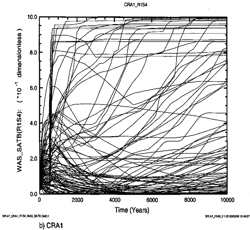
Figure 6-36. Brine saturation (dimensionless) in the waste panel versus time (years) for all 100 vectors in Replicate 1, Scenario S4. Figure a) shows results from the CRA-2004 PABC. Figure b) shows results from the CRA-2004.
