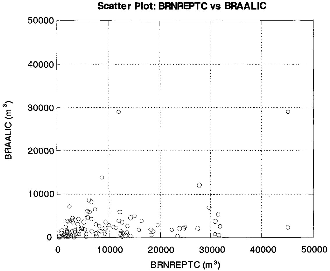
Figure 6-5. Scatter plot of total cumulative brine flow (m 3 ) into the DRZ versus cumulative brine flow (m 3 ) into the repository for all 100 vectors in Replicate 1, Scenario S1, CRA-2004 PABC.
