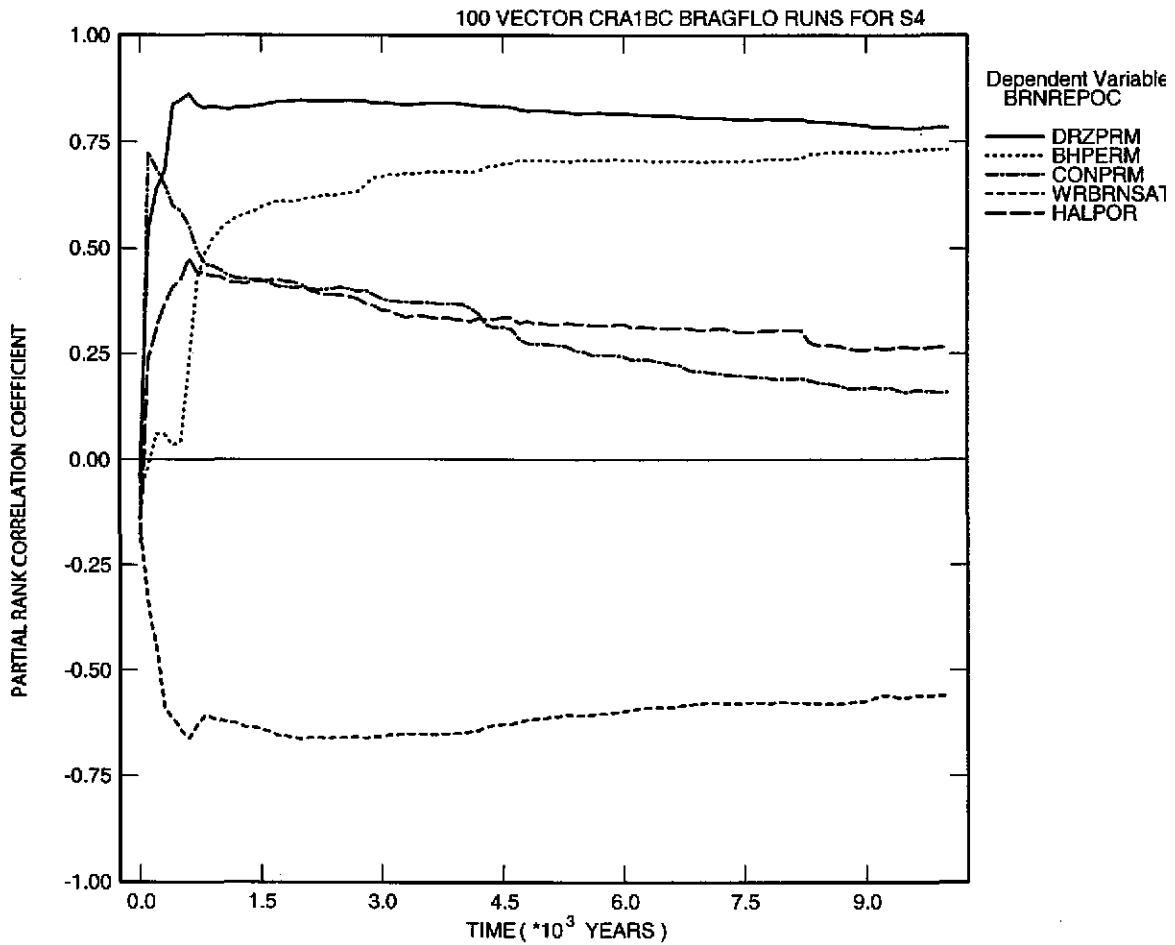
Figure 6-76. Primary correlations (dimensionless) of brine flow out of the repository with input parameters versus time (years) from the CRA-2004 PABC Replicate 1, Scenario S4. Table 4-2 gives a description of the names in the legend.
