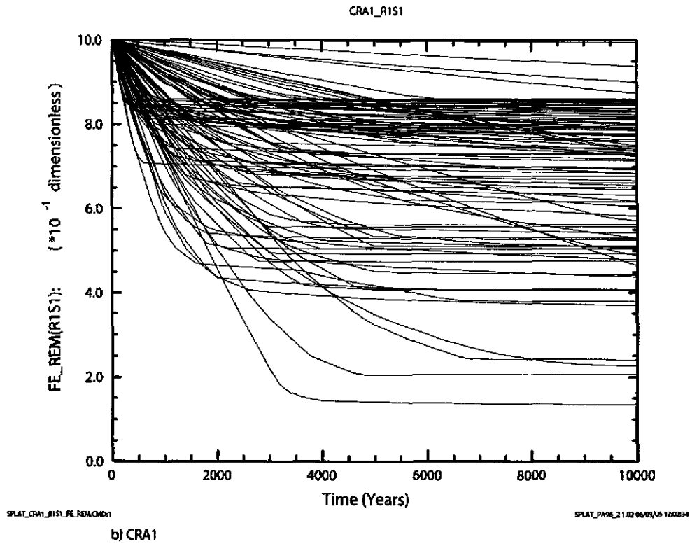
Figure 6-10. Fraction of iron (dimensionless) remaining versus time (years) for all 100 vectors in Replicate 1, Scenario S1. Figure a) shows results from the CRA-2004 PABC. Figure b) shows results from the CRA-2004.
