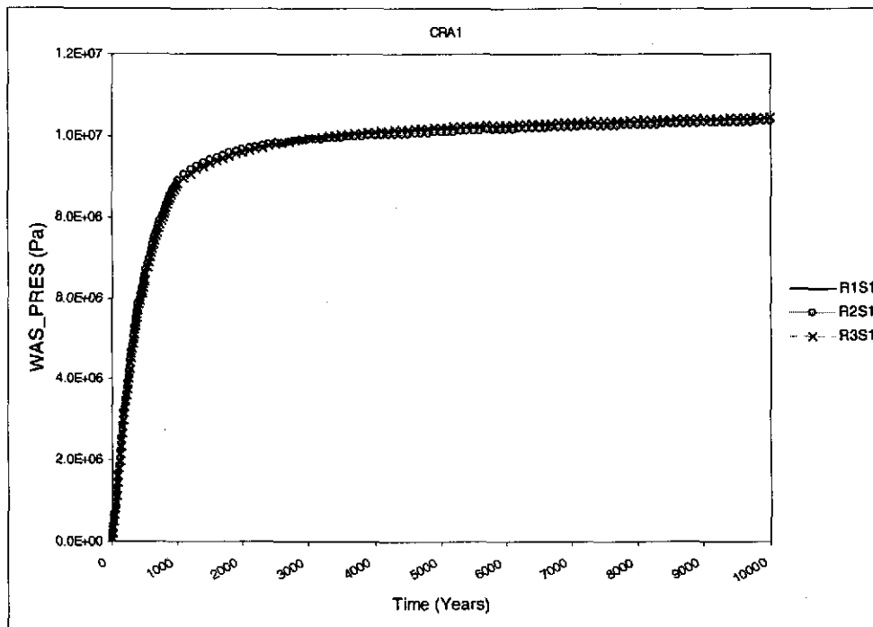
Figure 6-82. Volume averaged pressure (Pa) in the waste area versus time (years) from the CRA-2004 PABC, Scenario S1, Replicates 1-3.
