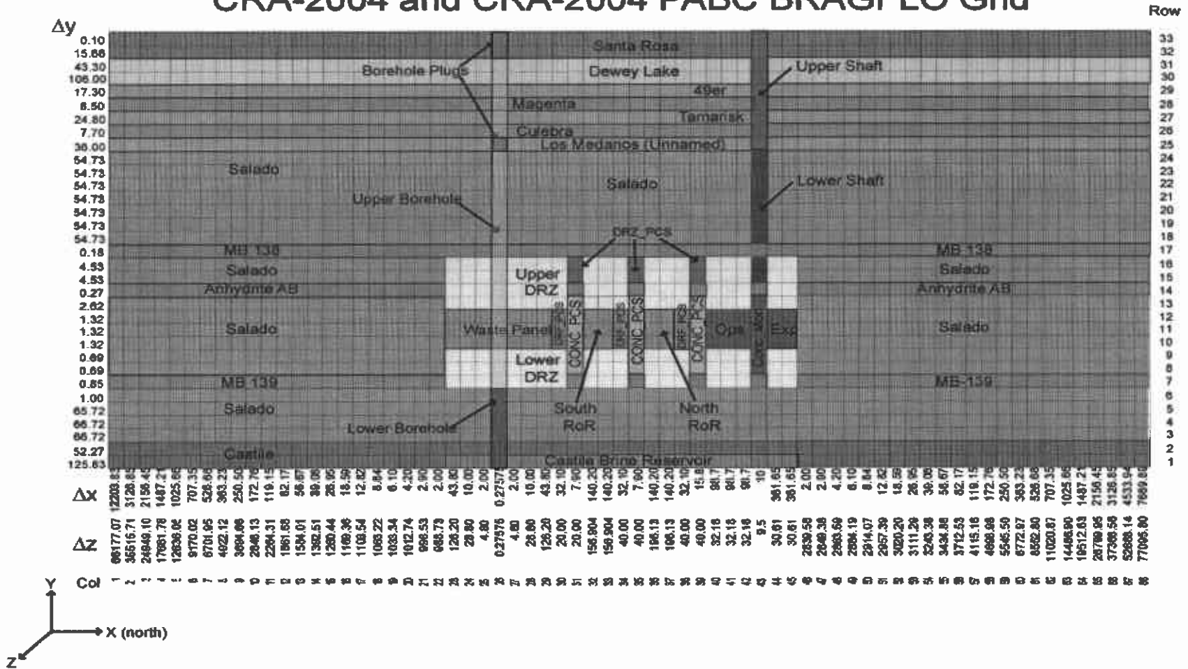
Figure 3-1. CRA-2004 PABC BRAGFLO grid ( \Delta x , \Delta y , and \Delta z dimensions in meters). Note that “north of the repository” is to the right of the Exp area on the above graph and “south of the repository” is to the left of the Panel area.
