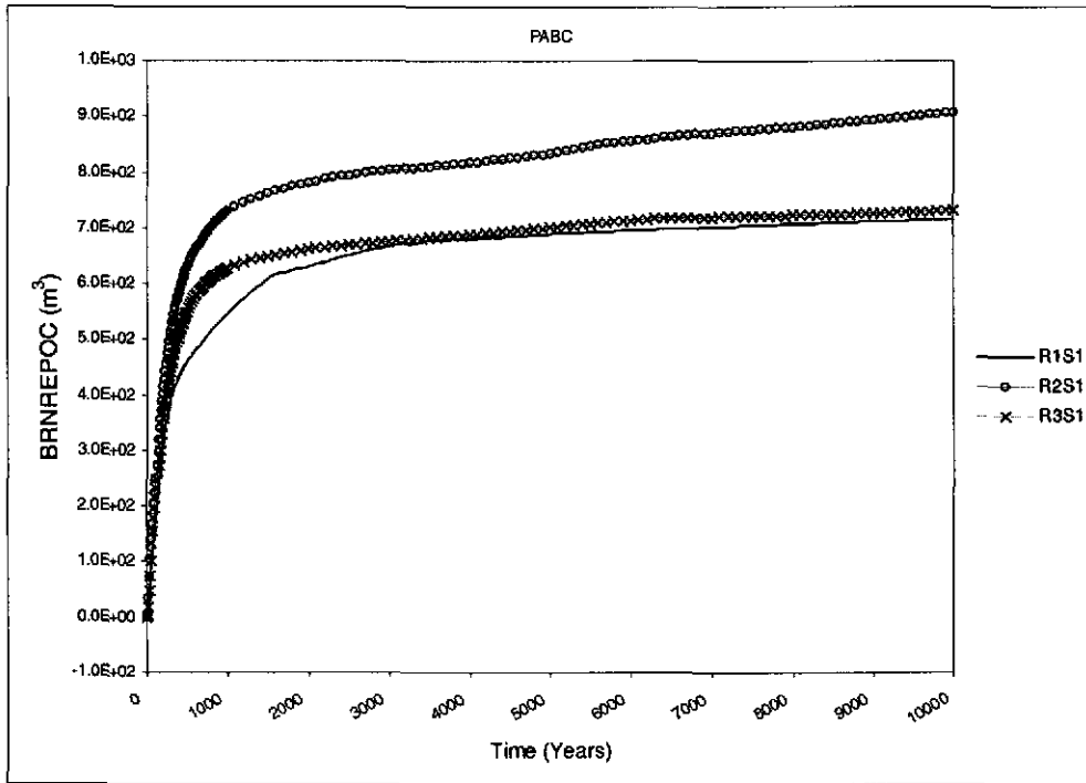
Figure 6-85. Cumulative brine flow ( m^3 ) away from the repository versus time (years) from the CRA-2004 PABC, Scenario S1, Replicates 1-3.
