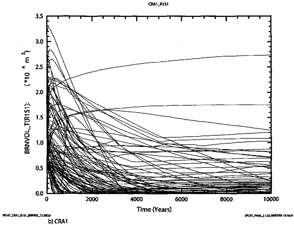
Figure 6-3. Total brine volume ( m^3 ) in all waste regions versus time (years) for all 100 vectors in Replicate 1, Scenario S1. Figure a) shows results from the CRA-2004 PABC. Figure b) shows results from the CRA-2004.
