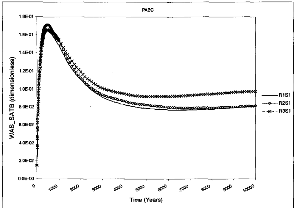
Figure 6-83. Volume-averaged brine saturation (dimensionless) in the waste panel versus time (years) from the CRA-2004 PABC, Scenario S1, Replicates 1-3. Note that brine saturation axis maximum is set at 0.18 to emphasize the differences.
