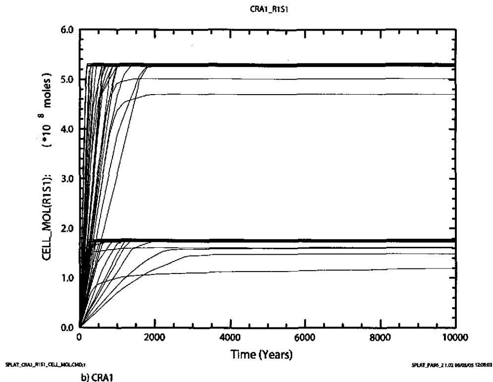
Figure 6-12. Cumulative gas generation (moles) due to microbial activity versus time (years) for all 100 vectors in Replicate 1, Scenario S1. Figure a) shows results from the CRA-2004 PABC. Figure b) shows results from the CRA-2004.
