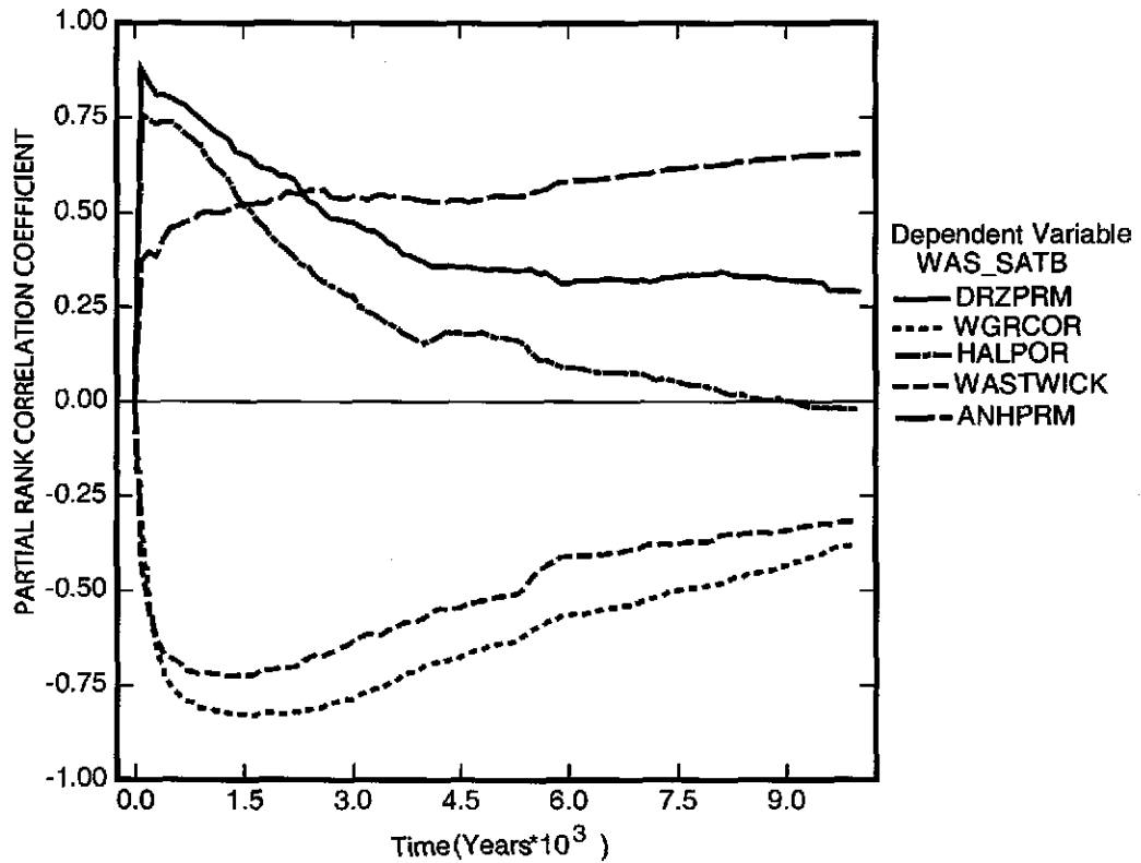
Figure 6-8. Primary correlations of brine saturation (dimensionless) in the waste panel with input parameters versus time (years), for Replicate 1, Scenario S1, CRA-2004 PABC. Table 4-2 gives a description of the names in the legend.
