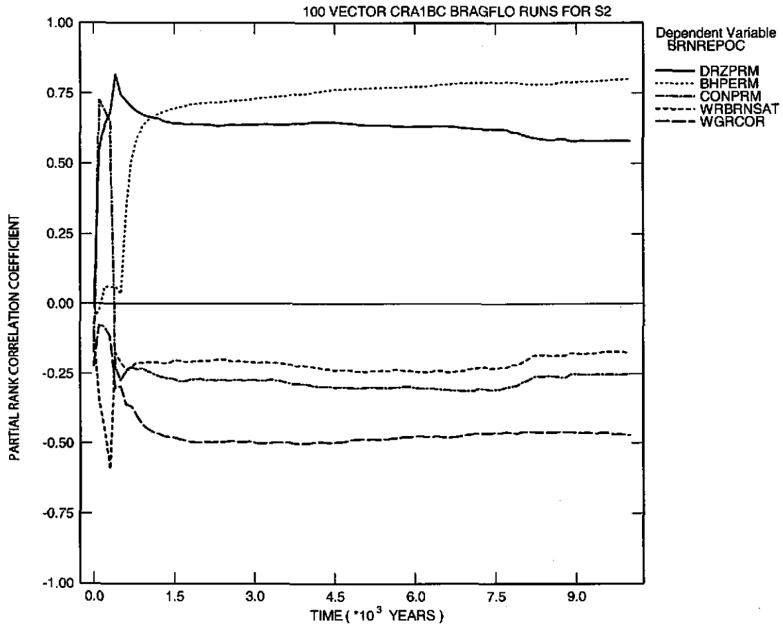
Figure 6-75. Primary correlations (dimensionless) of brine flow out of the repository with input parameters versus time (years) from the CRA-2004 PABC Replicate 1, Scenario S2. Table 4-2 gives a description of the names in the legend.
