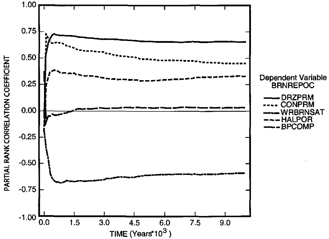
Figure 6-27. Primary correlations (dimensionless) of cumulative brine outflow from the repository with input parameters versus time (years) from the CRA-2004 PABC, Replicate 1, Scenario S1. Table 4-2 gives a description of the names in the legend.
