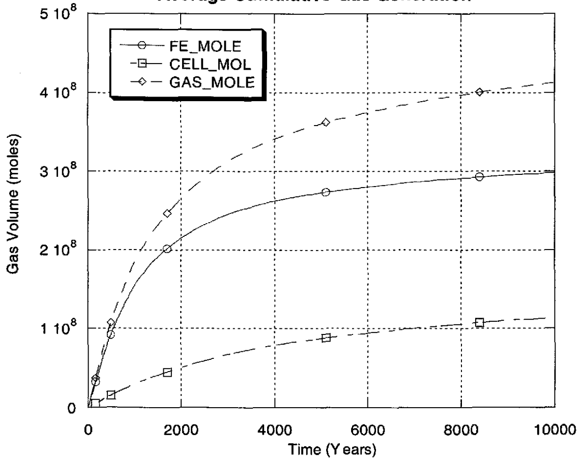
Figure 6-17. Cumulative gas generation (moles) by corrosion, by microbial activity and total versus time (years), averaged over 100 vectors from Replicate 1, Scenario S1 of the CRA-2004 PABC.
