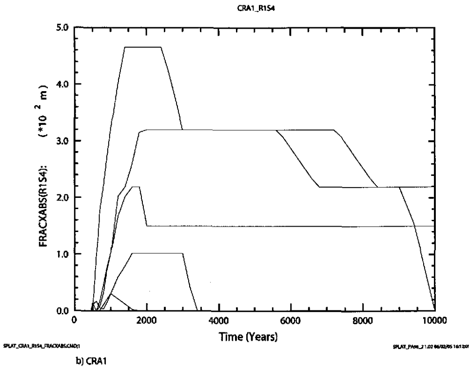
Figure 6-70. Fracture length (m) in Anhydrite A&B, south of the repository versus time (years) for all 100 vectors in Replicate 1, Scenario S4. Figure a) shows results from the CRA-2004 PABC. Figure b) shows results from the CRA-2004.
