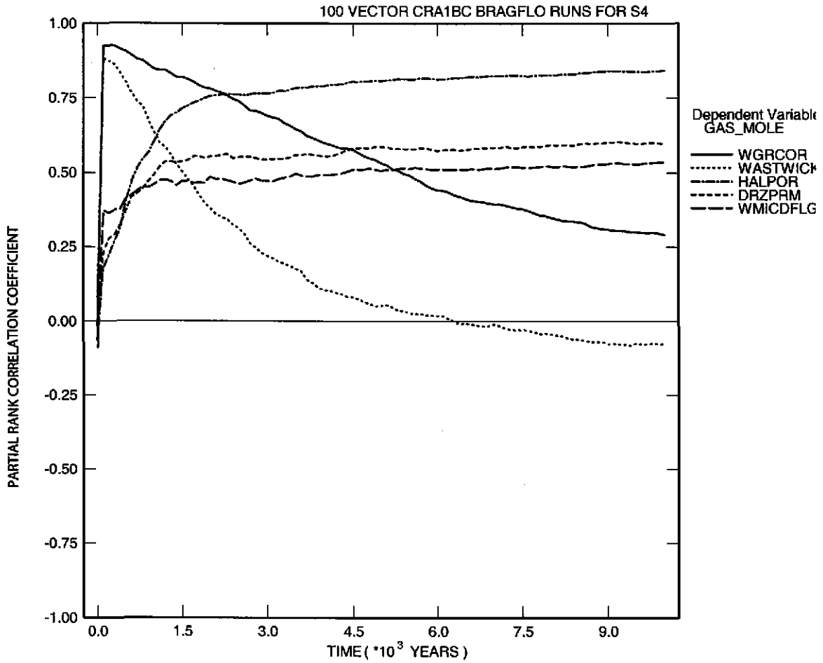
Figure 6-54. Primary correlations of cumulative amount (moles) of gas produced in the Waste Panel with input parameters, versus time (years) from the CRA-2004 PABC Replicate 1, Scenario S4. Table 4-2 gives a description of the names in the legend.
