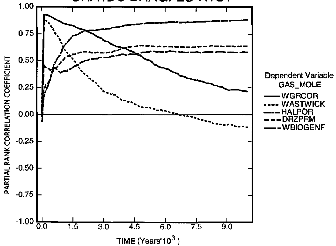
Figure 6-16. Primary correlations (dimensionless) of cumulative microbial gas generation with input parameters versus time (years) from the CRA-2004 PABC, Replicate 1, Scenario S1. Table 4-2 gives a description of the names in the legend.
