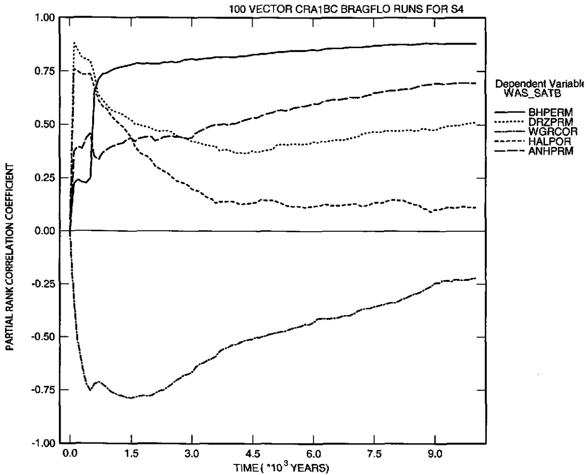
Figure 6-38. Primary correlations of brine saturation (dimensionless) in the waste panel with input parameters versus time (years) from the CRA-2004 PABC, Replicate 1, Scenario S4. Table 4-2 gives a description of the names in the legend.
