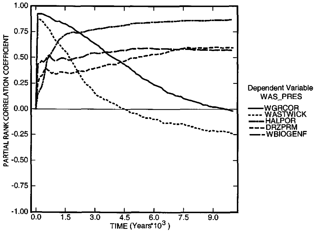
Figure 6-19. Primary correlations (dimensionless) of volume averaged pressure in the waste area with input parameters versus time (years) from the CRA-2004 PABC, Replicate 1, Scenario S1. Table 4-2 gives a description of the names in the legend.
