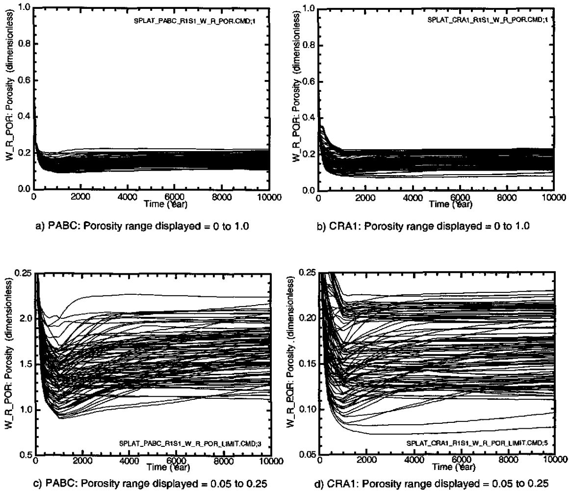
Figure 6-1. Volume averaged porosity (dimensionless) in all waste regions versus time (years) for all 100 vectors in Replicate 1, Scenario S1. Figures a) and c) show results from the CRA-2004 PABC. Figures b) and d) show results from the CRA-2004.
