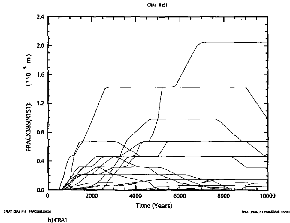
Figure 6-21. Fracture length (m) in MB138 south of the repository versus time (years) for all 100 vectors in Replicate 1, Scenario S1. Figure a) shows results from the CRA-2004 PABC. Figure b) shows results from the CRA-2004.
