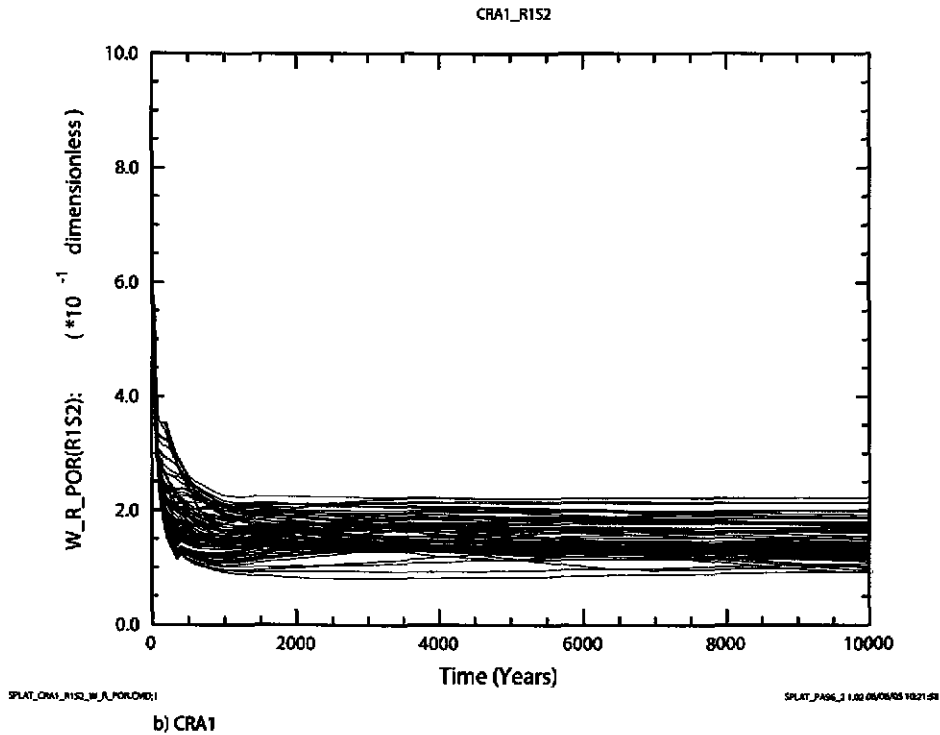
Figure 6-29. Volume averaged porosity (dimensionless) in all waste regions versus time (years) for all 100 vectors in Replicate 1, Scenario S2. Figure a) shows results from the CRA-2004 PABC. Figure b) shows results from the CRA-2004.
