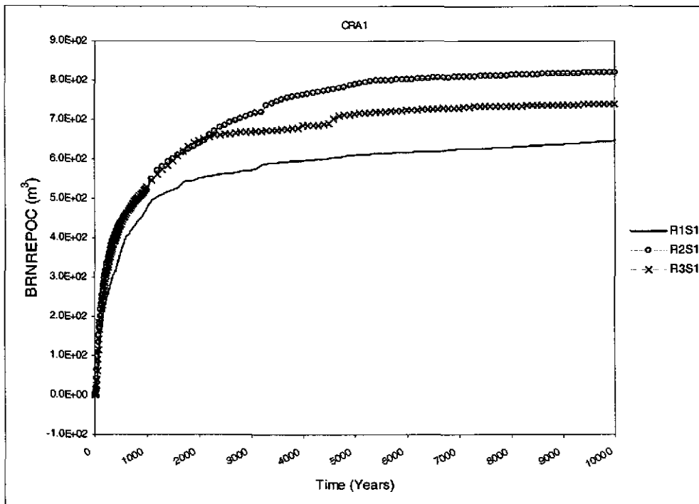
Figure 6-86. Cumulative brine flow ( m^3 ) away from the repository versus time (years) from the CRA-2004 PABC, Scenario S1, Replicates 1-3.
