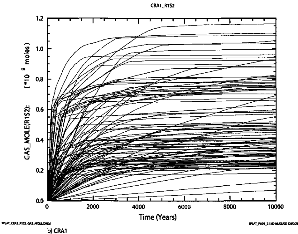
Figure 6-51. Total cumulative amount of gas (moles) generated versus time (years) for all 100 vectors in Replicate 1, Scenario S2. Figure a) shows results from the CRA-2004 PABC. Figure b) shows results from the CRA-2004.
