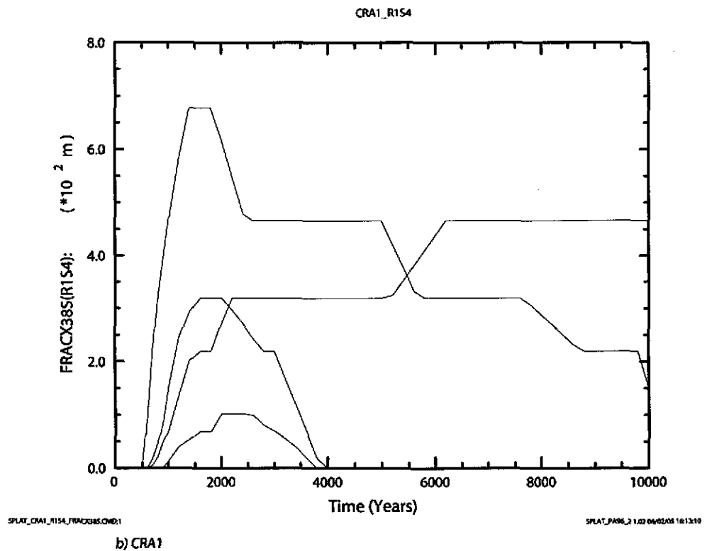
Figure 6-62. Fracture length (m) in MB138, south of the repository versus time (years) for all 100 vectors in Replicate 1, Scenario S4. Figure a) shows results from the CRA-2004 PABC. Figure b) shows results from the CRA-2004.
