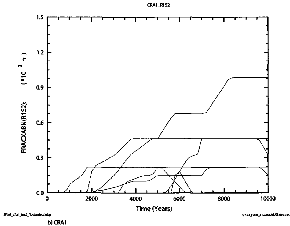
Figure 6-67. Fracture length (m) in Anhydrite A&B, north of the repository versus time (years) for all 100 vectors in Replicate 1, Scenario S2. Figure a) shows results from the CRA-2004 PABC. Figure b) shows results from the CRA-2004.
