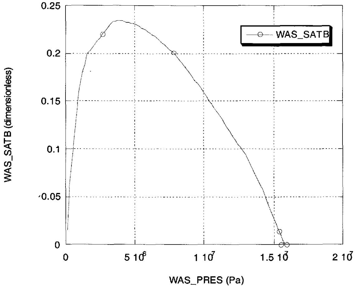
Figure 6-7. Brine saturation (dimensionless) in the waste panel versus pressure (Pa) in the waste panel for Vector 28, Replicate 1, Scenario S1, CRA-2004 PABC.
