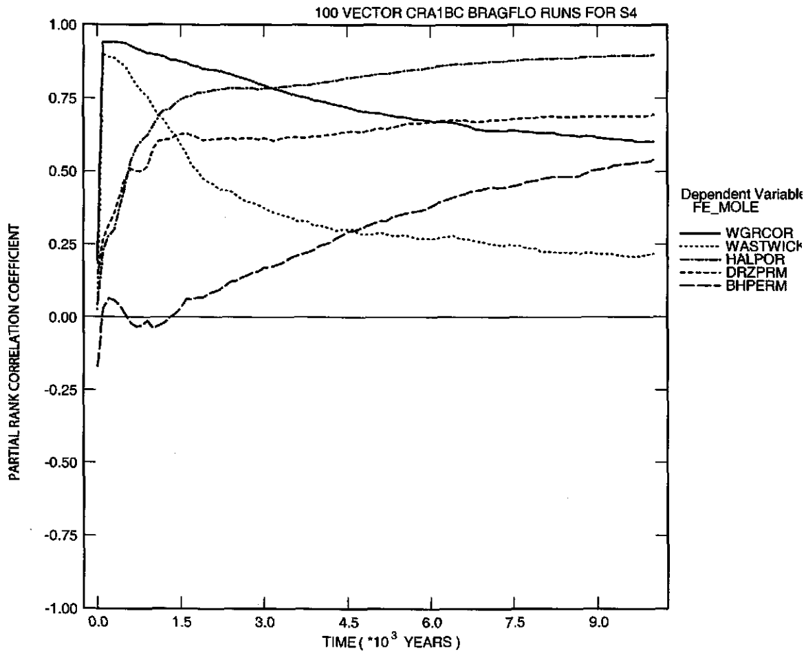
Figure 6-42. Primary correlations of cumulative amount (moles) of gas produced by iron corrosion in the waste panel with input parameters versus time (years) from the CRA-2004 PABC, Replicate 1, Scenario S4. Table 4-2 gives a description of the names in the legend.
