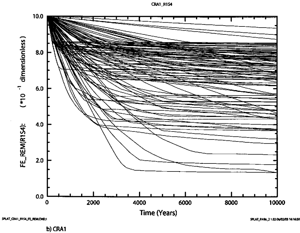
Figure 6-44. Fraction of iron (dimensionless) remaining versus time (years) for all 100 vectors in Replicate 1, Scenario S4. Figure a) shows results from the CRA-2004 PABC. Figure b) shows results from the CRA-2004.
