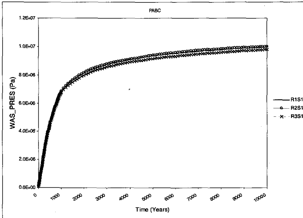
Figure 6-81. Volume averaged pressure (Pa) in the waste area versus time (years) from the CRA-2004 PABC, Scenario S1, Replicates 1-3.
