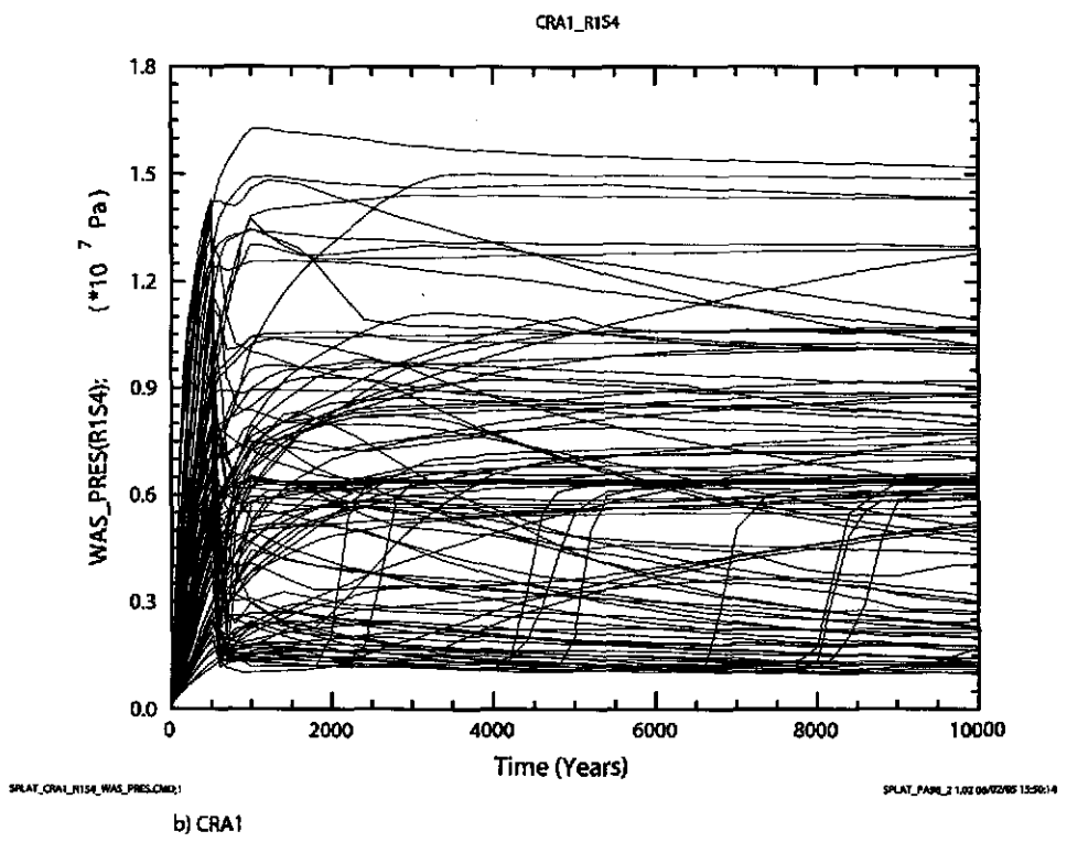
Figure 6-56. Volume averaged pressure (Pa) in the waste area versus time (years) for all 100 vectors in Replicate 1, Scenario S4. Figure a) shows results from the CRA-2004 PABC. Figure b) shows results from the CRA-2004.
