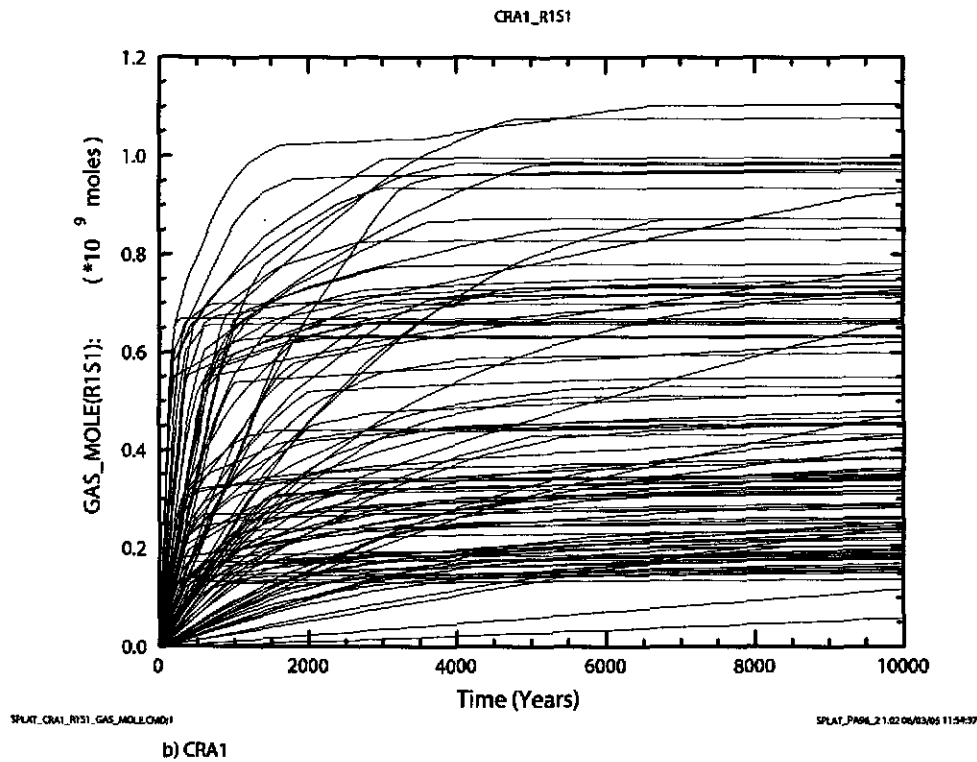
Figure 6-15. Cumulative gas generation (moles) by all processes versus time (years) for all 100 vectors in Replicate 1, Scenario S1. Figure a) shows results from the CRA-2004 PABC. Figure b) shows results from the CRA-2004.
