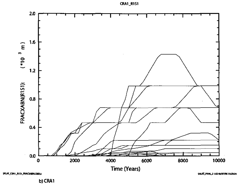
Figure 6-24. Fracture length in Anhydrite A&B (m) north of the repository versus time (years) for all 100 vectors in Replicate 1, Scenario S1. Figure a) shows results from the CRA-2004 PABC. Figure b) shows results from the CRA-2004.
