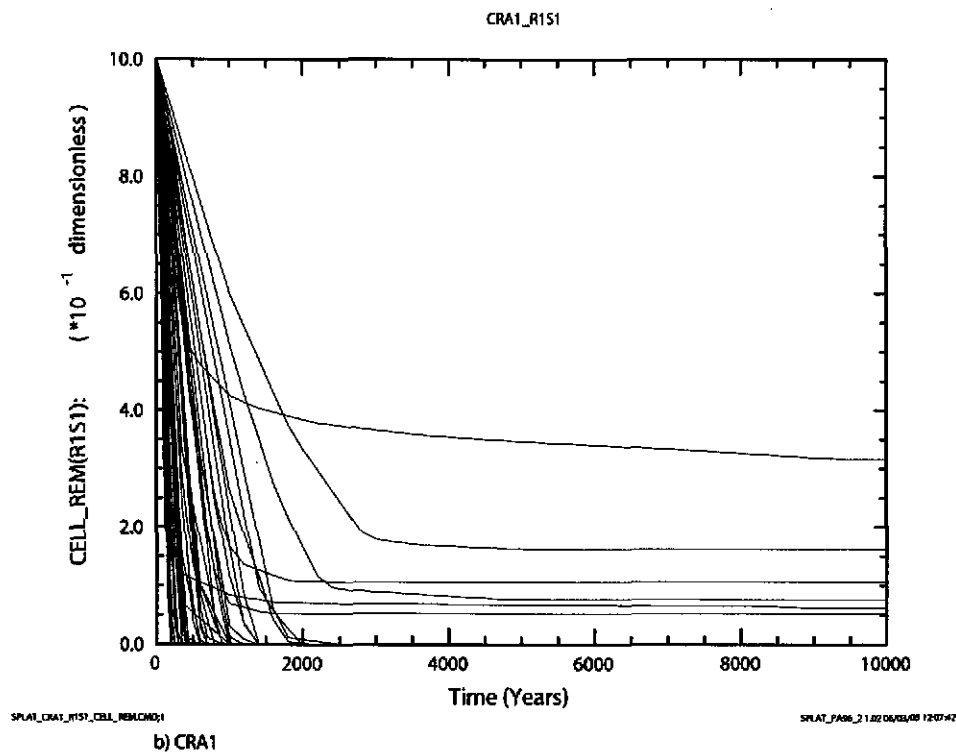
Figure 6-13. Remaining fraction of cellulose (dimensionless) versus time (years) for all 100 vectors in Replicate 1, Scenario S1. The remaining fraction of cellulose is either cellulose or CPR depending on the value of WAS_AREA:PROBDEG (§5.4). Figure a) shows results from the CRA-2004 PABC. Figure b) shows results from the CRA-2004.
