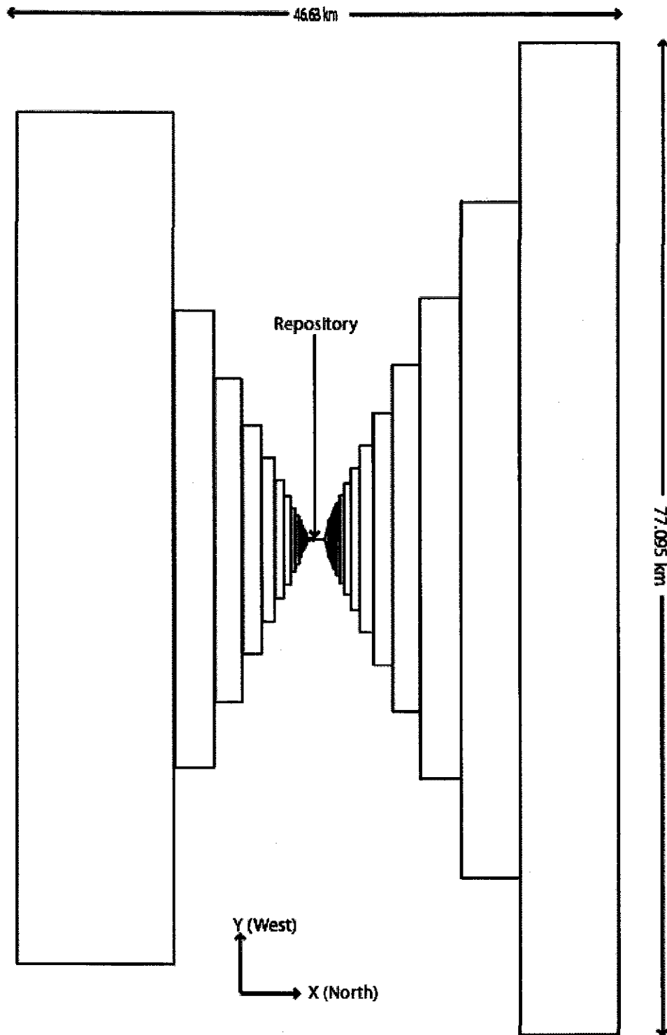
Figure 3-2. Top view of CRA-2004, CRA-2004 PABC logical grid showing the radial flaring.
