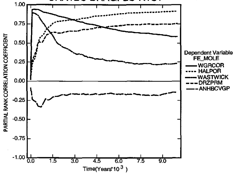
Figure 6-11. Primary correlations (dimensionless) of cumulative gas generation by corrosion with input parameters versus time (years) from the CRA-2004 PABC, Replicate 1, Scenario S1. Table 4-2 gives a description of the names in the legend.
