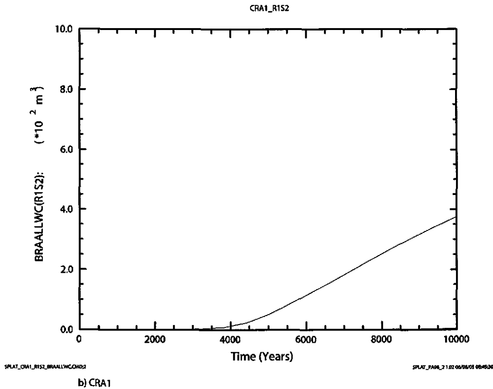
Figure 6-79. Cumulative brine flow ( m^3 ) to the LWB versus time (years) for all 100 vectors in Replicate 1, Scenario S2. Figure a) shows results from the CRA-2004 PABC. Figure b) shows results from the CRA-2004.
