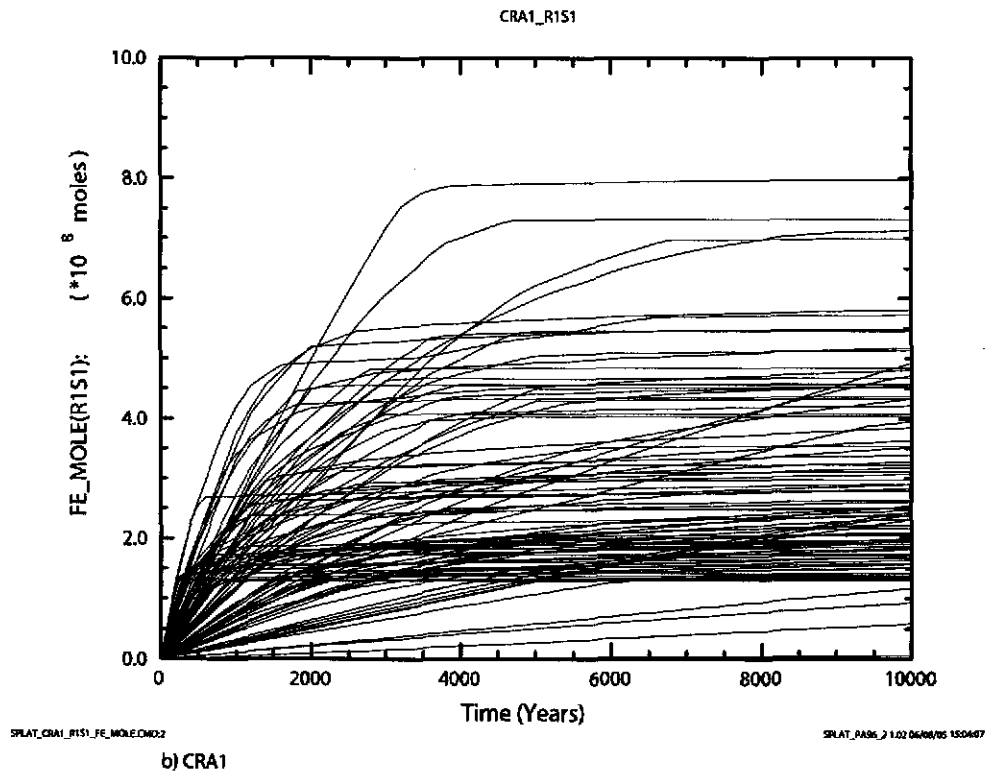
Figure 6-9. Cumulative gas generation (moles) by iron corrosion versus time (years) for all 100 vectors in Replicate 1, Scenario S1. Figure a) shows results from the CRA-2004 PABC. Figure b) shows results from the CRA-2004.
