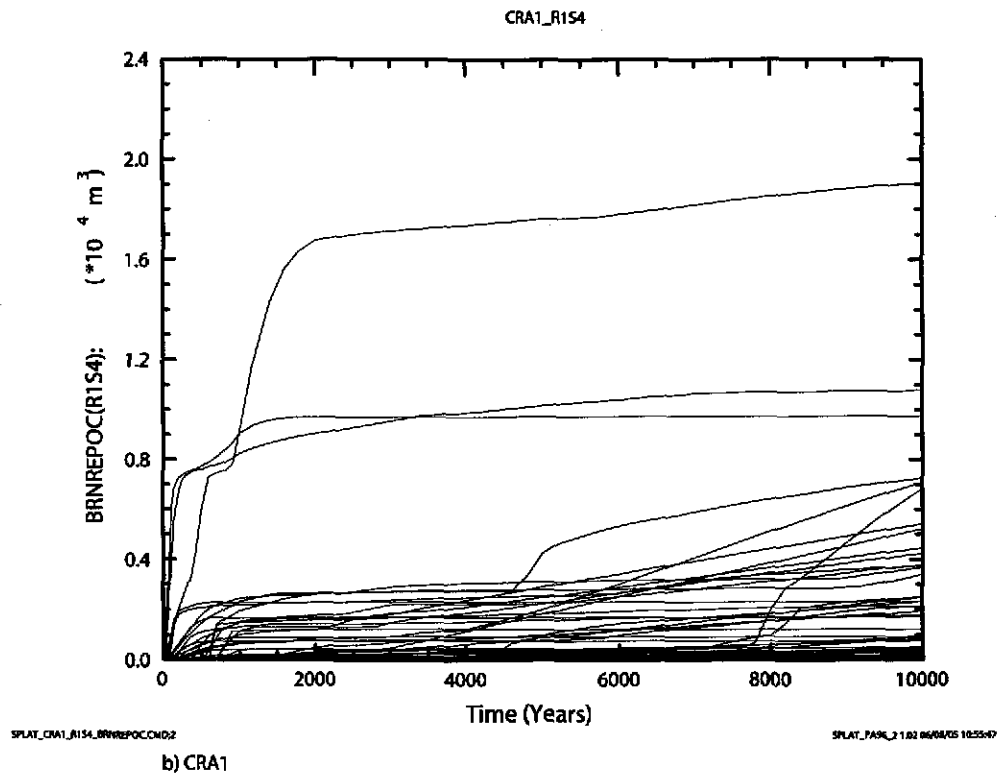
Figure 6-74. Cumulative brine flow ( m^3 ) out of the repository versus time (years) for all 100 vectors in Replicate 1, Scenario S4. Figure a) shows results from the CRA-2004 PABC. Figure b) shows results from the CRA-2004.
