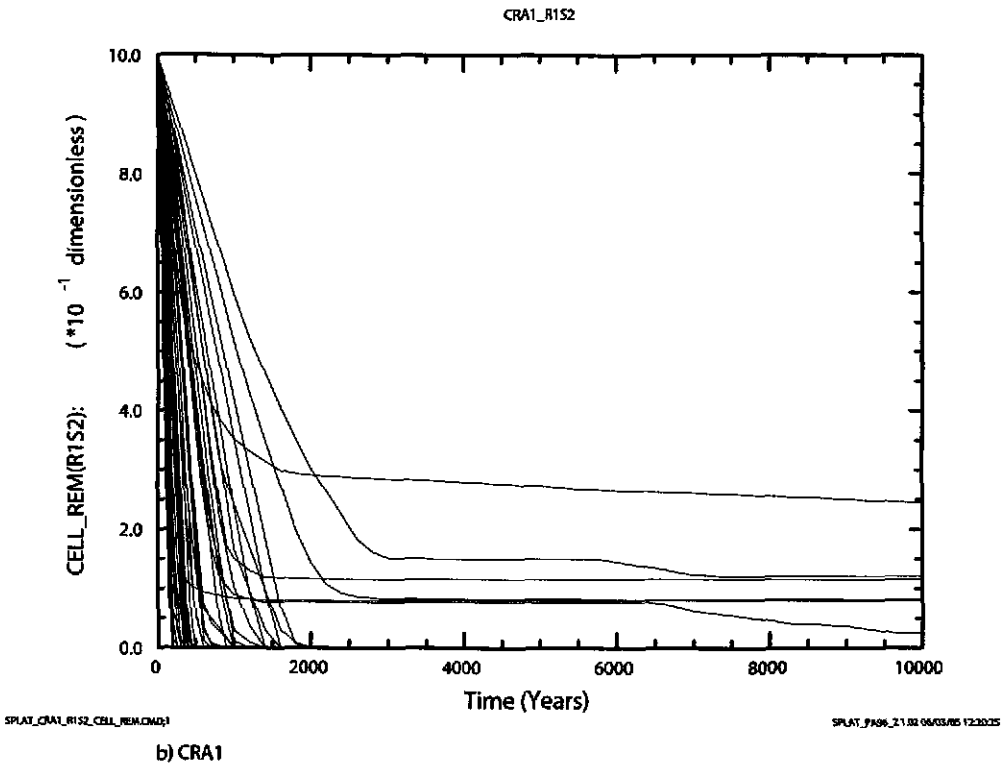
Figure 6-49. Fraction of cellulose (dimensionless) remaining versus time (years) for all 100 vectors in Replicate 1, Scenario S2. Fraction of cellulose is either cellulose or CPR depending on the value of WAS_AREA:PROBDEG (see §5.4). Figure a) shows results from the CRA-2004 PABC. Figure b) shows results from the CRA-2004.
