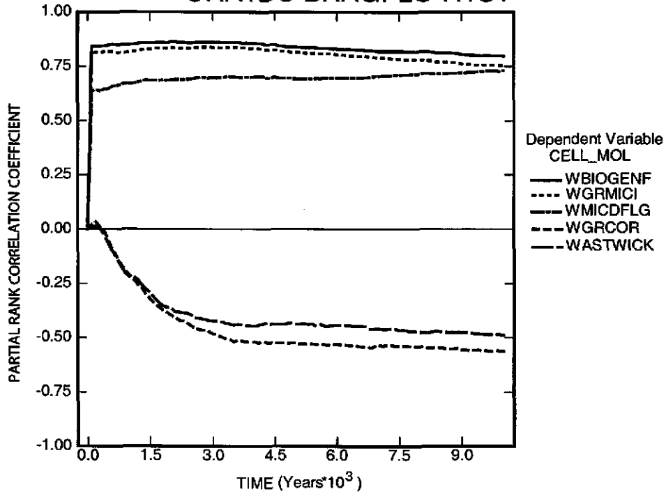
Figure 6-14. Primary correlations (dimensionless) of cumulative microbial gas generation with input parameters versus time (years), from the CRA-2004 PABC, Replicate 1, Scenario S1, CRA-2004 PABC. Table 4-2 gives a description of the names in the legend.
