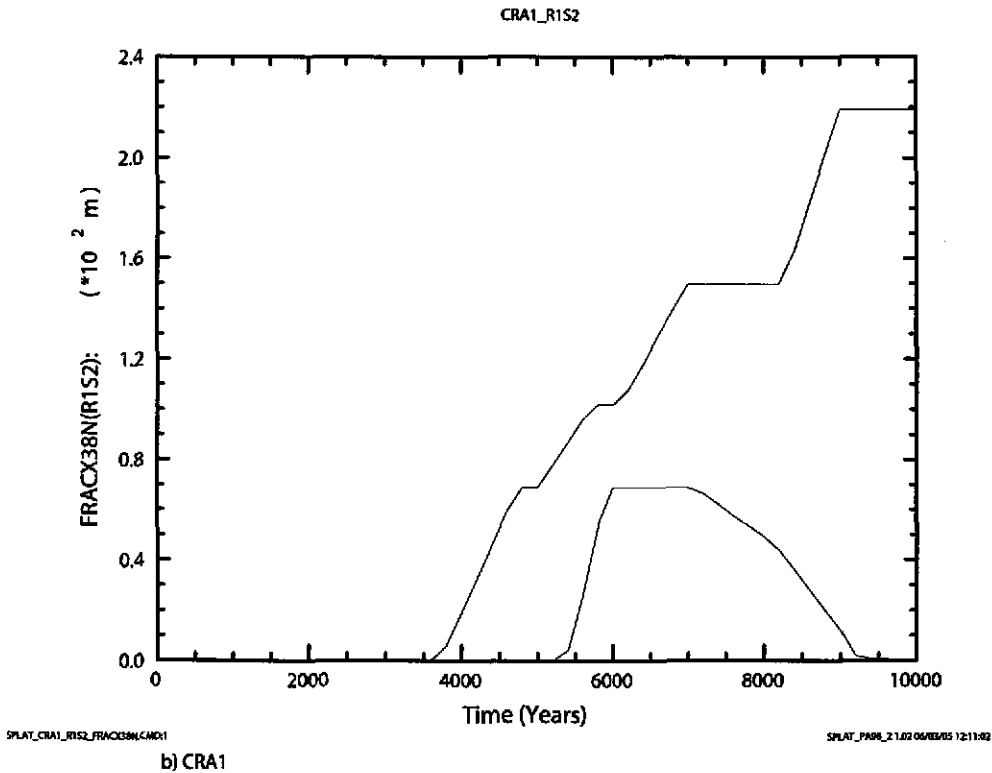
Figure 6-59. Fracture length (m) in MB138, north of the repository versus time (years) for all 100 vectors in Replicate 1, Scenario S2. Figure a) shows results from the CRA-2004 PABC. Figure b) shows results from the CRA-2004.
