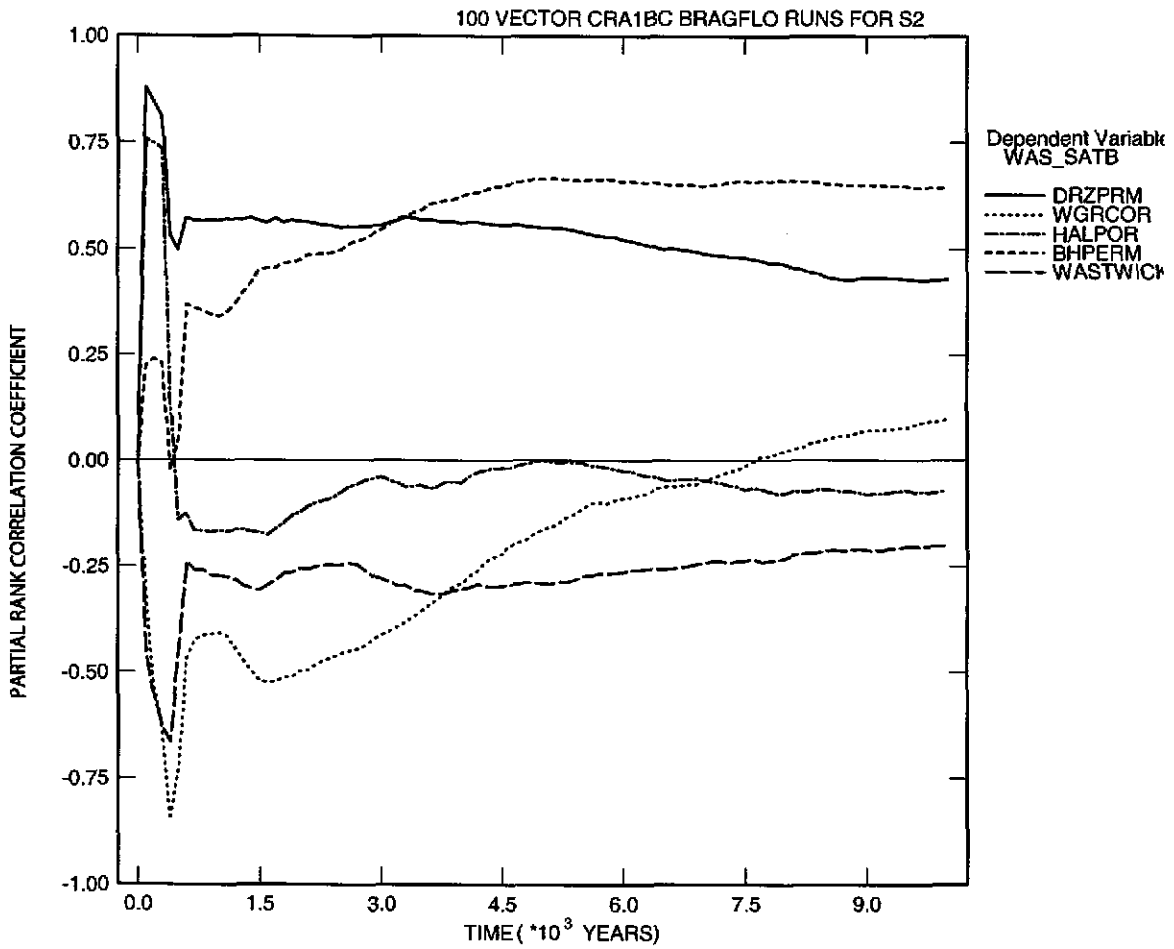
Figure 6-37. Primary correlations of brine saturation (dimensionless) in the Waste Panel with input parameters versus time (years) from the CRA-2004 PABC, Replicate 1, Scenario S2. Table 4-2 gives a description of the names in the legend.
