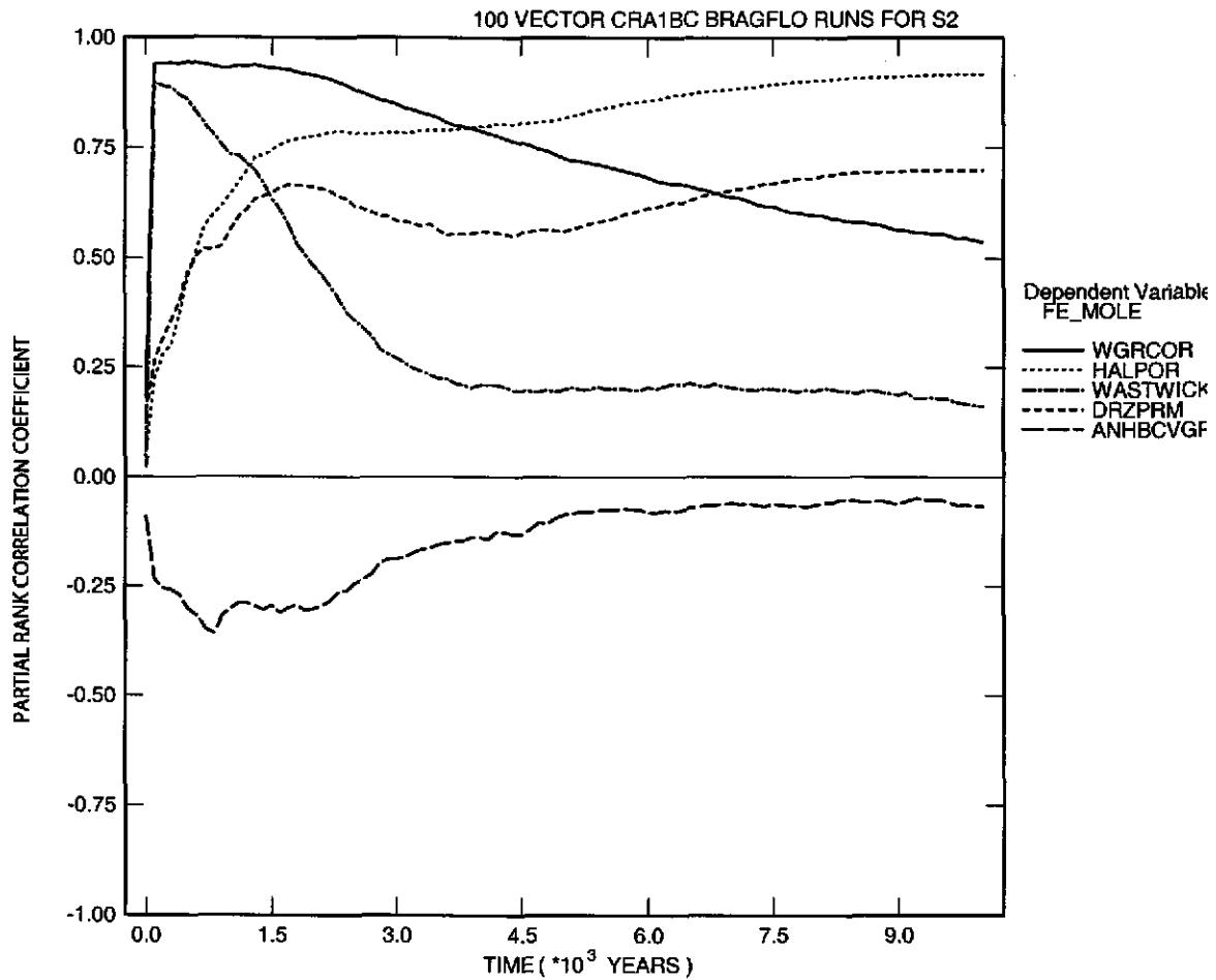
Figure 6-41. Primary correlations of cumulative amount (moles) of gas produced by iron corrosion in the waste panel with input parameters versus time (years) from the CRA-2004 PABC, Replicate 1, Scenario S2. Table 4-2 gives a description of the names in the legend.
